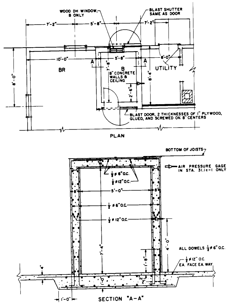
Fig. 10—Plan and section of concrete bathroom shelter.
